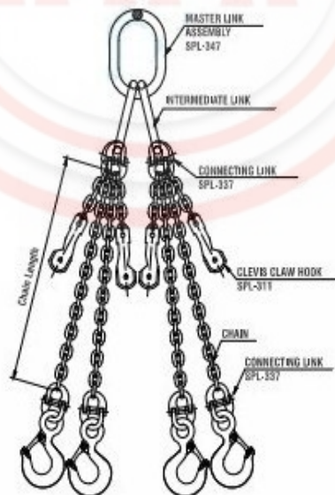
Four Leg Chain Sling SLC-46S
