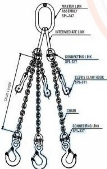
Three Leg Chain Sling SLC-45S
