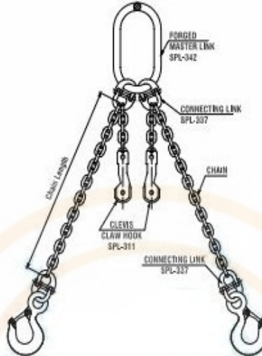
Tow Leg Chain Sling SLC-44S
